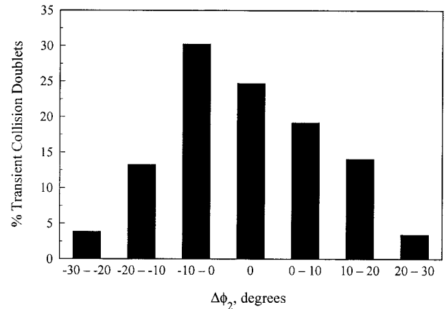
FIGURE 3 Histogram of the differential distribution in \Delta\phi_2 of transient collision doublets at G = 110 s -1 binned into intervals of 10^\circ , N = 303 . 74% of the doublets lie in the interval -30^\circ < \Delta\phi_2 < +30^\circ .
