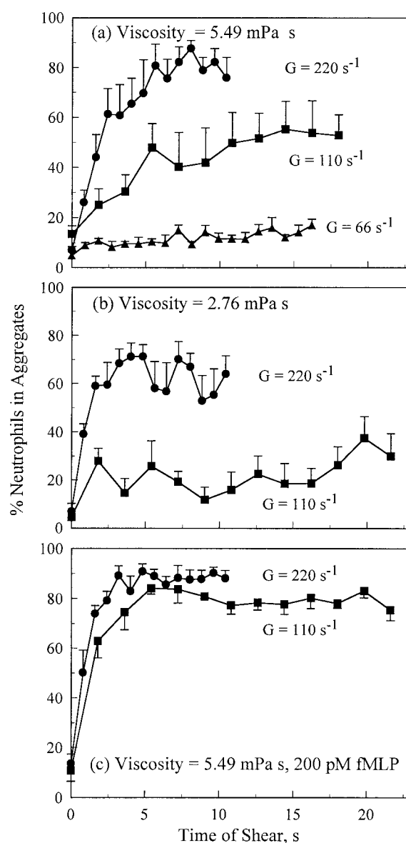
FIGURE 5 Effect of shear rate and shear stress on the rate of neutrophil aggregation in (a) 10% Ficoll at G = 66, 110 , and 220 \text{ s}^{-1} ; (b) 5% Ficoll at G = 110 and 220 \text{ s}^{-1} ; (c) 10% Ficoll with neutrophils preincubated for 3 min with 200 pM fMLP. Plot of the mean fraction of neutrophils in aggregates ( \pm \text{SEM} , n = 5 ) against time of shear. There was a marked rise in the rate and extent of aggregation with increasing shear rate and a significant reduction in the extent of aggregation in 5% Ficoll at the lower shear stress. The chemotactically stimulated cells exhibited a significant increase in the rate and extent of aggregation.
